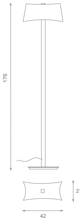
Pie de salon/Column Ref.62016 2 E27 60w
