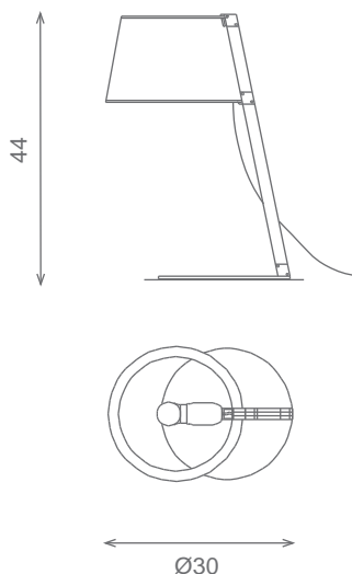
Sobremesa/Table lamp Ref.61003 1 E27 60w
