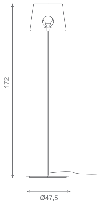
Pie de salon/Column Ref.62009 💡1 E27 G120 100w
