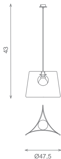
Suspension/Hanging lamp Ref.60012 💡1 E27 G120 100w
