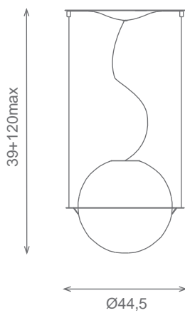
Suspension/Hanging lamp Ref.60011 💡 1 E27 60w
