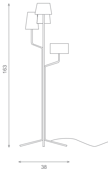
Pie de salon/Column Ref.62025 💡4 E14-60w
